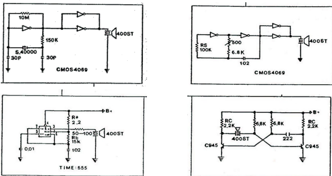
SUGGESTED OSCILLATING CIRCUITS
